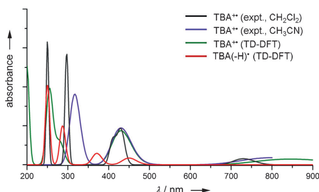
Figure 1. Absorption spectra of TBA •+ and neutral aminyl radical TBA(–H) • . The spectra were reconstructed by digitizing the spectra displayed in Refs. [2,3].
